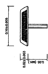
SIDE ELEVATION OF ROAD STUD NOT TO SCALE
