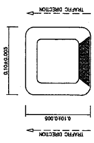
PLAN OF UNI-DIRECTIONAL TYPE ROAD STUD NOT TO SCALE
